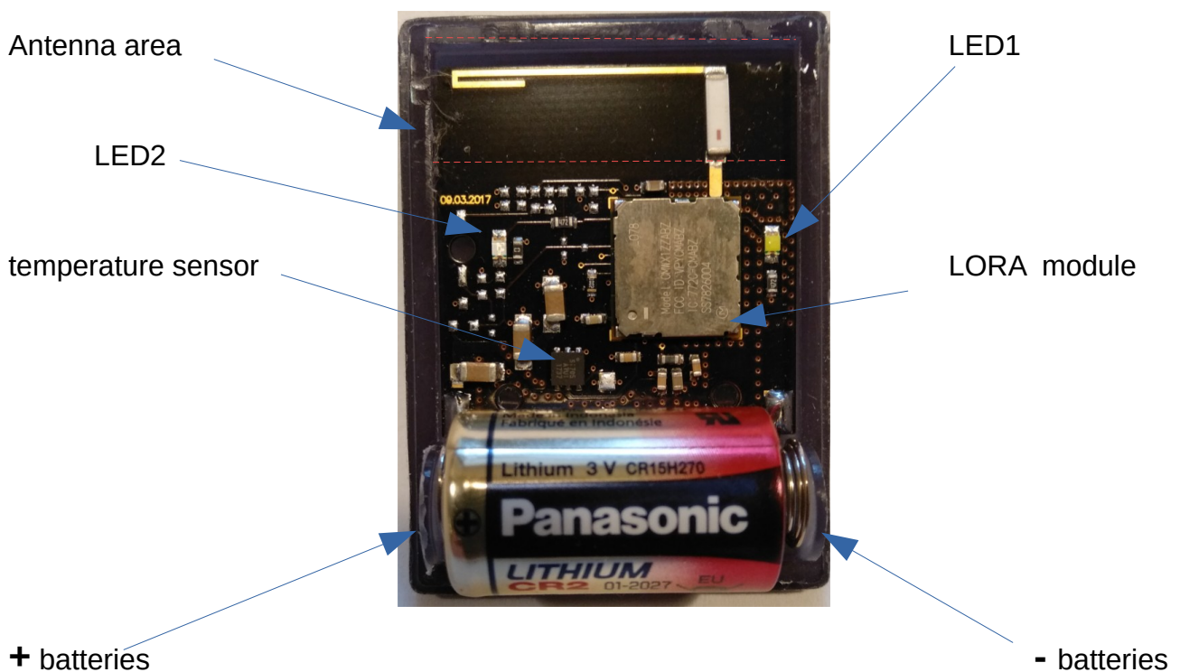
iNode LORA T – view after removing the cover
